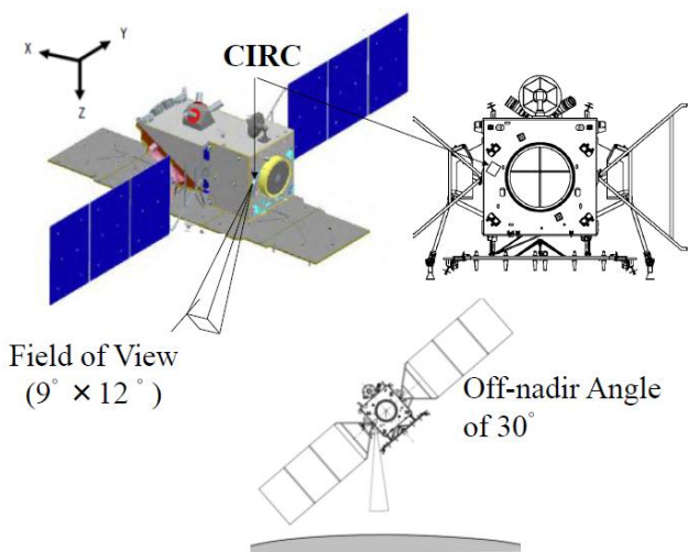
Fig. 2 Schematic view of ALOS-2
