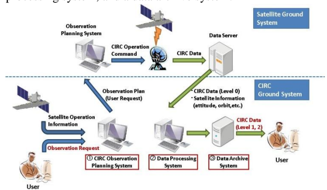
Fig. 5 Overview of ALOS-2/CIRC Ground System (ACGS)
