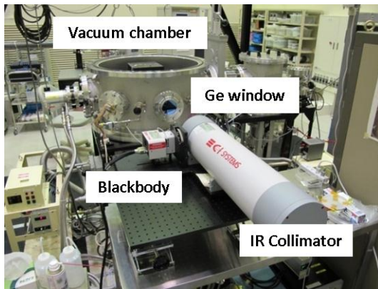
Fig. 7 Experimental setup of MTF measurement
