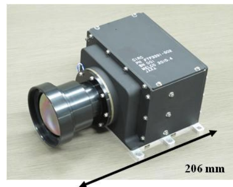
Fig. 11 CIRC Ground Test Model (GTM)
