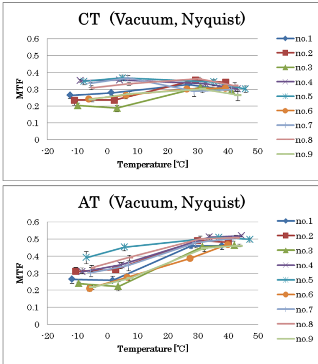
Fig. 10 Measurement results of MTF. MTF in the CT direction (top). MTF in the AT direction (bottom)
