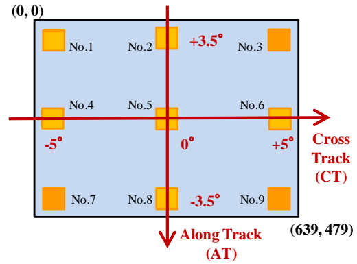
Fig. 8 Measurement points of MTF on image acquired by CIRCs
