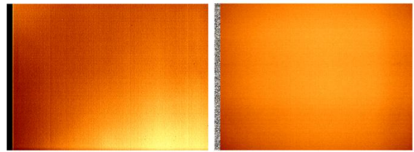
Fig. 11 Left image is a raw image of blackbody of CIRC. Right one is a corrected image of left one.
