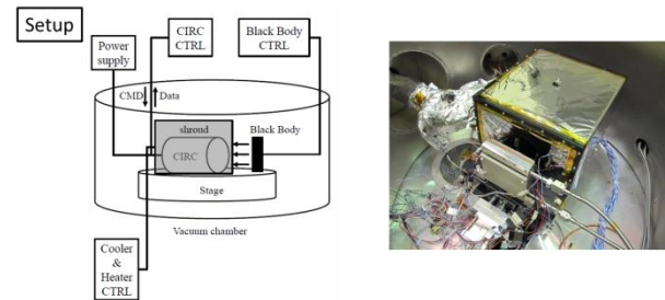
Fig. 9 Experimental setup for radiometric measurements
