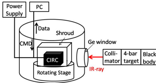
Fig. 6 Schematic view of MTF measurement
